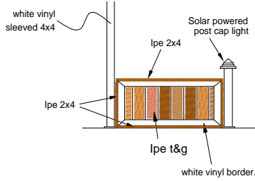
Ipe Shadow Box Exterior (Not to Scale)
