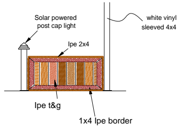
Ipe Shadow Box Interior (Not to Scale)
