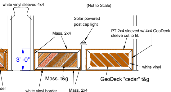
As we do for a Screen Porch "knee wall" (Not to Scale)
